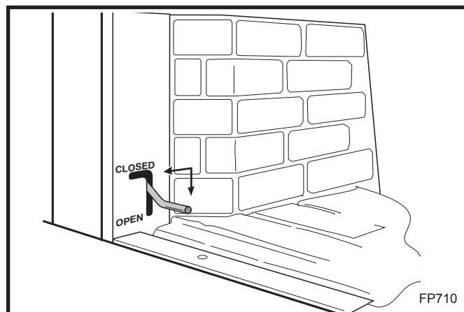
Fig. 7 Outside air operation.
